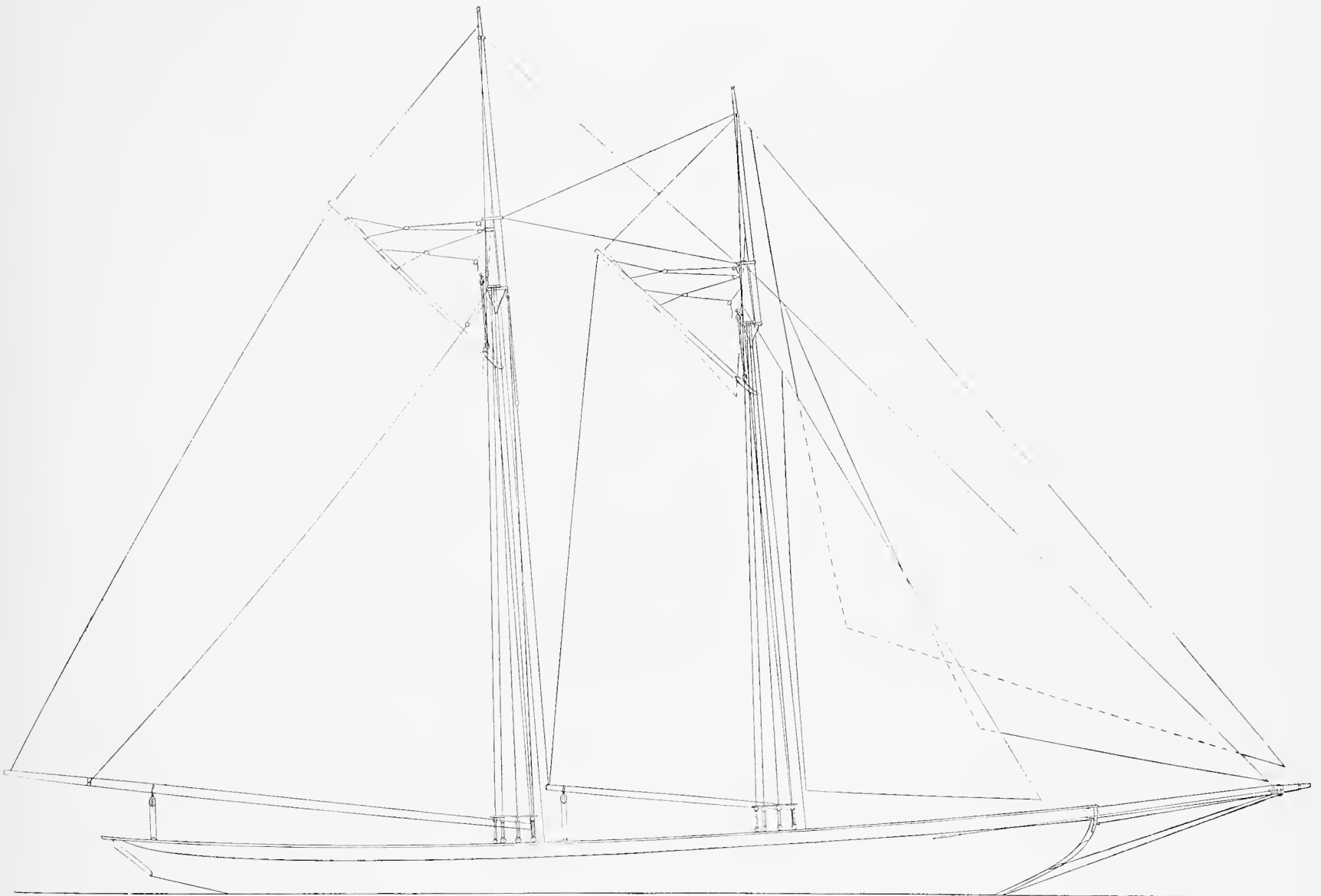
SAIL PLAN OF A MODERN PILOT BOAT.—Designed by A. Cary Smith, of New York, for Capt. T. B. Lasserre, of Fernandina, Fla.
